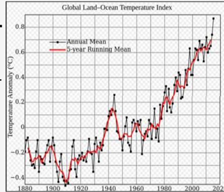
Grafik ©: https://data.giss.nasa.gov/gistemp/graphs_v3/fig_A2.gif
